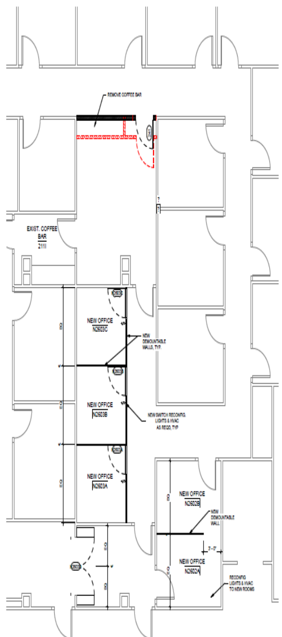
NEW OFFICES & BREAK ROOM ENLARGED ② PLAN 1/4" = 1'-0"
