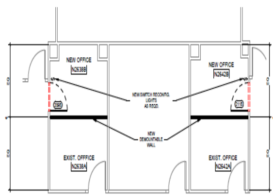
NEW OFFICES ENLARGED PLAN ① PLAN 1/4" = 1'-0"
